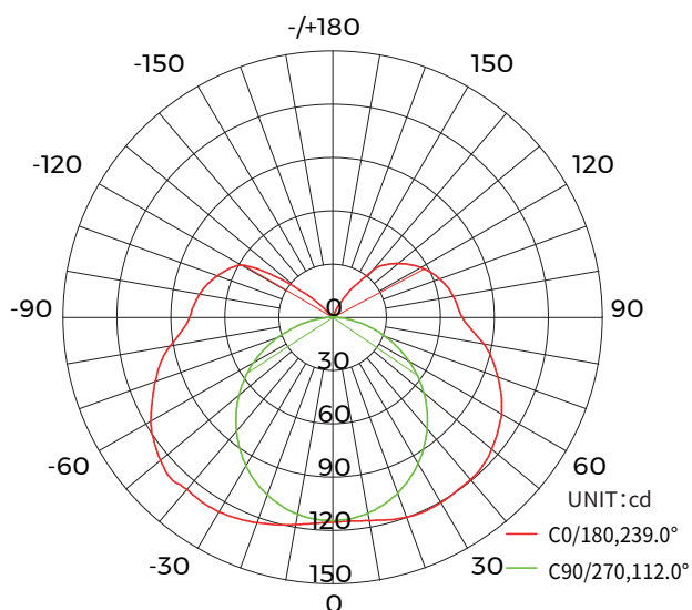
Light distribution
