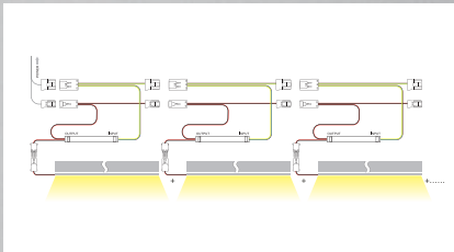
Integrated Track Cabling: Integrated track cabling solution, save effort and time, includes dimming and non-dimming.
