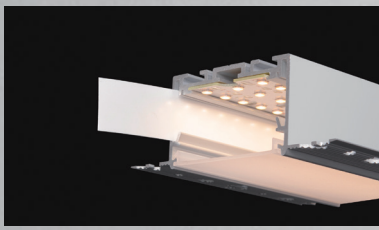
Luminous efficiency improved: Reflective paper is attached on the flanks of the profile, which can optimize and improve the luminous efficiency, and meet higher lighting requirements.
