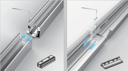
Interconnection of profile: New-added interconnection accessory of profile, the screws can be turned from the front of profile, convenient and efficient.
