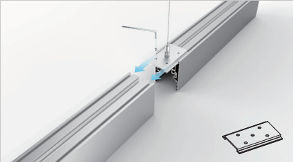
Interconnection of luminaire: The brand-new interconnection accessory, interconnection of the luminaire without disassembly, convenient and efficient.
