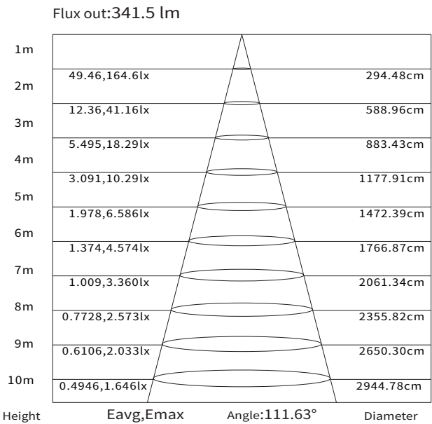
Effective average illuminance
