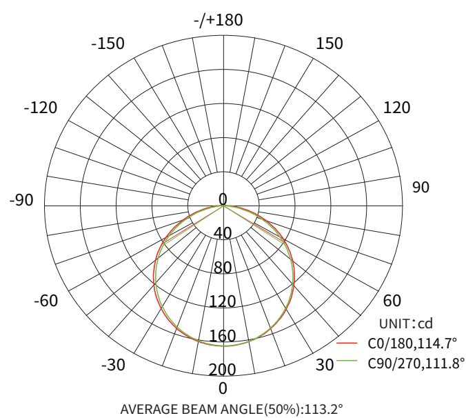
Light distribution
